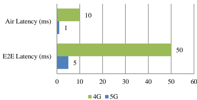
Figure 1 - Latency levels between 4G and 5G systems [30]
